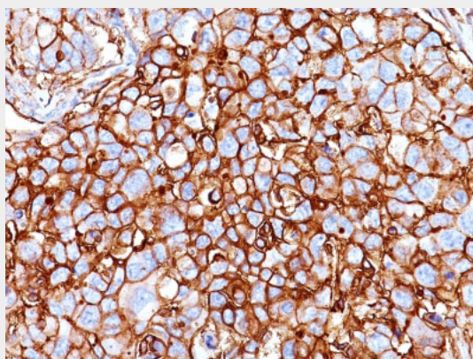
Formalin-fixed, paraffin-embedded human Breast Carcinoma stained with CD44 Monoclonal Antibody (HCAM/918)
