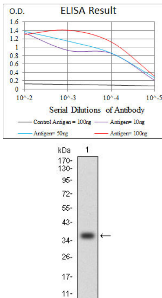
Figure 1: Western blot analysis using CCL2 mAb against human CCL2 (AA: 1-99) recombinant protein. (Expected MW is 36.5 kDa)
