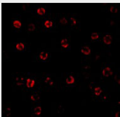
Immunofluorescence of Caspase-1 in HeLa cells with Caspase-1 antibody at 20 \mu\text{g/mL} .
