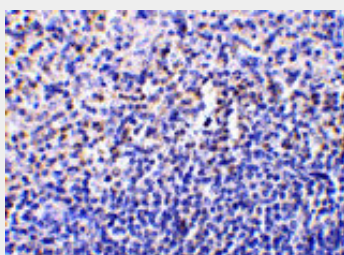
Immunohistochemistry of caspase-1 in human spleen tissue with caspase-1 antibody at 10 \mu\text{g/mL} .
