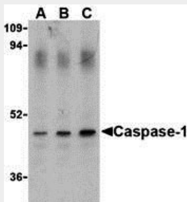
Western blot analysis of Caspase-1 in HeLa cell lysate with Caspase-1 antibody (IN) at (A) 0.5, (B) 1, and (C) 2 \mu\text{g/mL} .
