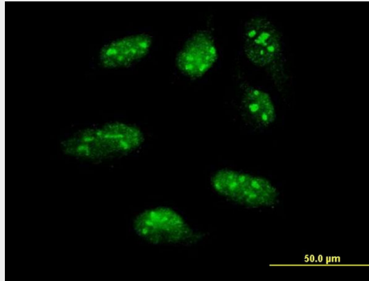
Immunofluorescence of monoclonal antibody to LHX1 on HeLa cell . [antibody concentration 10 ug/ml]
