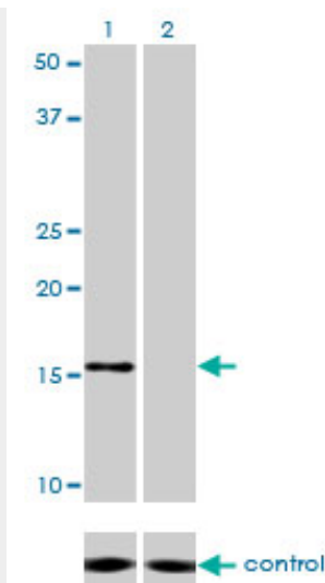
Western blot analysis of NDUFB7 over-expressed 293 cell line, cotransfected with NDUFB7 Validated Chimera RNAi (Cat # AT3005a)
