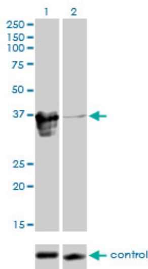
Western blot analysis of ZFP36L1 over-expressed 293 cell line, cotransfected with ZFP36L1 Validated Chimera RNAi (Cat # AT4574a)
